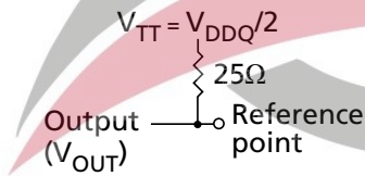
Figure 16: Output Slew Rate Load
