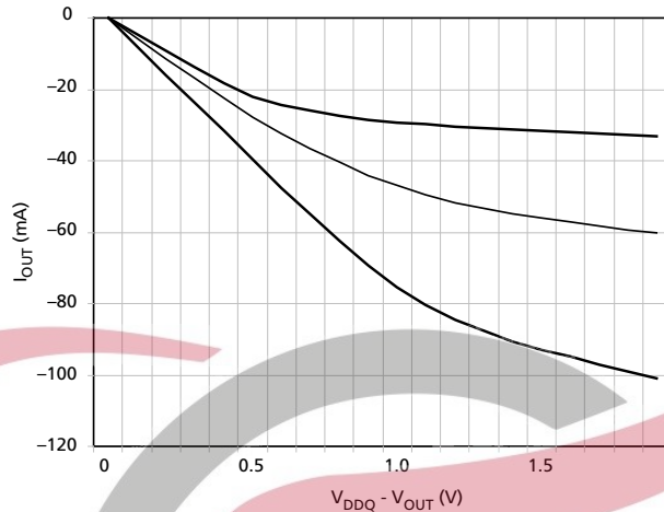
Figure 18: Full Strength Pull-Up Characteristics
